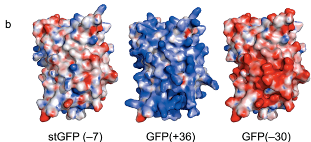
Figure 1. Supercharged green fluorescent proteins (GFPs). (a) Protein sequences of GFP variants, with fluorophore-forming residues highlighted green, negatively charged residues highlighted red, and positively charged residues highlighted blue. (b) Electrostatic surface potentials of the starting GFP (stGFP), GFP- (+36) , and GFP- (-30) , colored from -25 kT/e (red) to +25 kT/e (blue).
